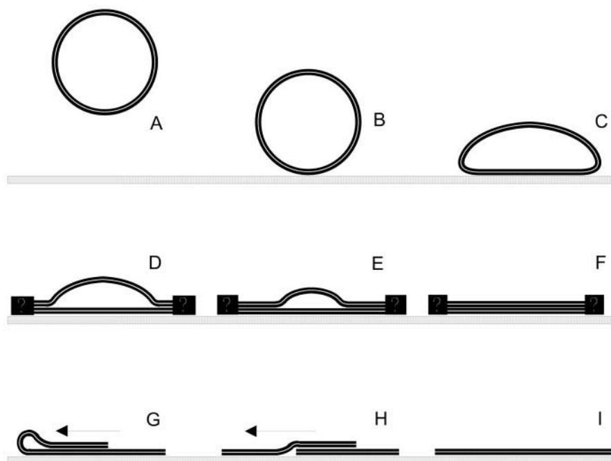
FIGURE 5 A simple and unified interpretation of the transformation from liposome to supported planar bilayer as suggested by the AFM sequences. The liposome approaches ( A ), adsorbs ( B ), and attaches ( C ) to a surface. As attached, it begins to flatten from the edges ( D ). The outer, flattened areas expand and spread ( E ), resulting into a partially flattened liposome ( D and E ). The liposome collapses to form two bilayers ( F ) stacked on top of each other. The uppermost bilayer moves from the lower one to unoccupied areas on the surface. This movement can occur by two mechanisms, rolling as in G and sliding as in H , in both cases resulting in a single bilayer structure ( I ). The edges are marked as boxes, as the AFM images are not clear enough to give information about the structure and organization at the boundaries. The edge-to-edge effects between adjacent membrane structures, which might be a requisite for the process or at least speeds it up considerably, are not included in this simplified scheme.
