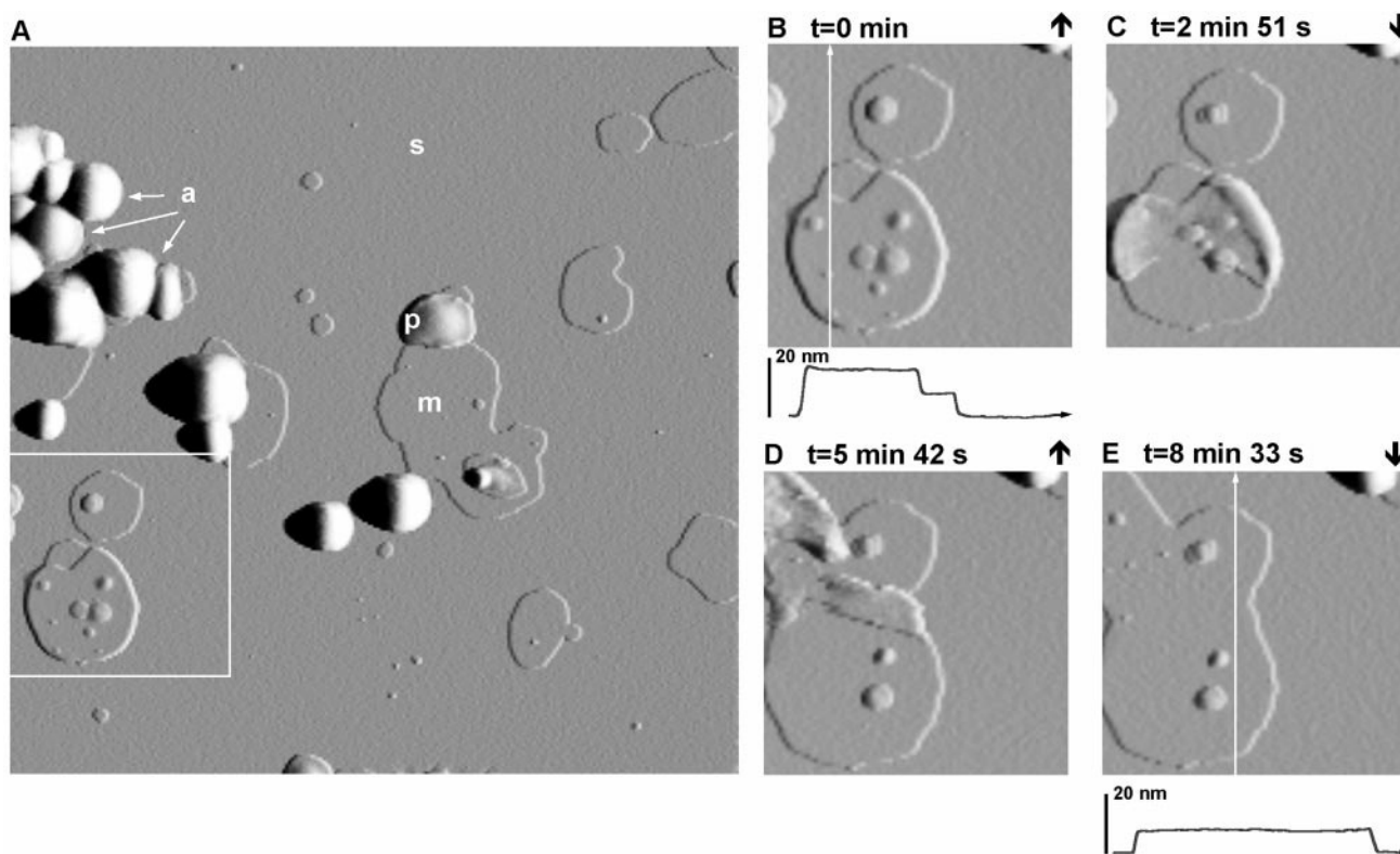
FIGURE 2 AFM sequence capturing the intermediate states during planar bilayer formation from glycolipid-containing liposomes on a hydrophilic silica surface. The images are collected in Tris-HCl/NaCl buffer and presented in the amplitude mode; however, cross sections and measurements are done in the height mode. This sequence shows the top bilayer of a flattened liposome collapsed and moving over the bottom bilayer before it produces a single confluent lipid membrane. ( A ) A 10- \mu m scan shows a number of different stages of the process, including attached liposomes ( a ), partially flattened liposomes ( p ), and membrane disks ( m ) on the silica surface ( s ). The sequence in B through E occurs in the outlined box (3 \mu m \times 3 \mu m). The cross section in B shows that the disk is composed of two bilayers (7.8 nm each) on top of each other, with a total height of 16 nm. ( C and D ) The top layer moves over the bottom layer to the silica surface and coalesces to form the single bilayer structure seen in the cross section of E . The slow scan direction is indicated by the large arrows above each image.
